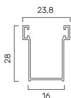
In allum. A16 16 x 28 mm GUAL..16M
