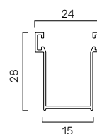
In allum. A14 15 x 28 mm GUAL..14M
