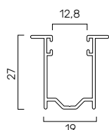
in allum. A26 19 x 27 mm GUAL..26M
