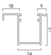
in allum. A31 24 x 31 mm GUAL..31M
