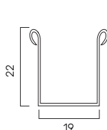
in ferro 19 x 22 mm GUFERSM
