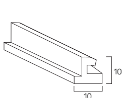
In gomma 10 x 10 mm TERPVCDU
